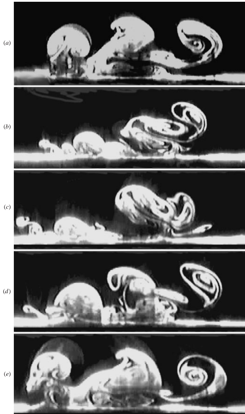
FIGURE 15. A sequence showing how quickly the vortex tubes undergo wrapping and unwrapping around each other during a single cycle. Note the striking similarity between (a) and (e) and the fact that for the K and \beta values under consideration the structures recover from a highly chaotic state only to start anew from a nearly identical initial state. Third facility, A = 29.5 mm, D = 355.6 mm, f = 1 Hz, K = 0.52 , \beta = 1.2 \times 10^5 .
